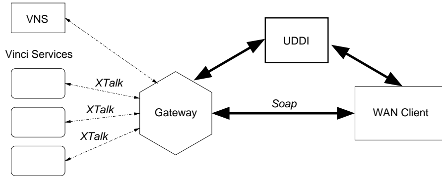
Fig. 6. Vinci services can be provided outside the local area using a protocol such as SOAP and a gateway.
